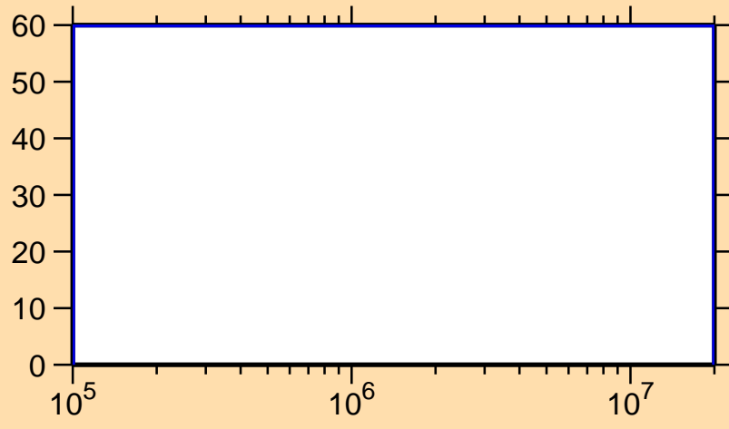
\Delta\sigma/\sigma vs. E for ^{119}\text{La}(n,n_1)
