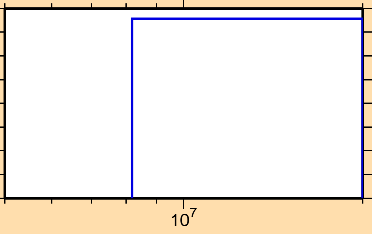
\sigma vs. E for ^{119}\text{La}(n,nt)
