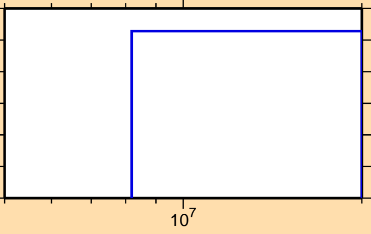
\sigma vs. E for ^{119}\text{La}(n,\text{nd})
