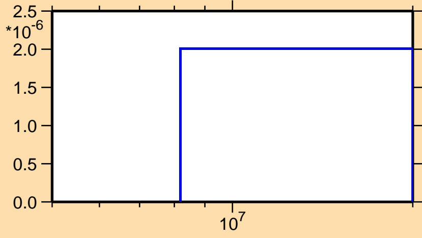
\sigma vs. E for ^{119}\text{La}(n,\text{pt})
