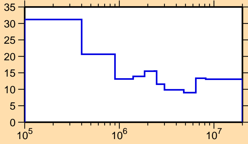
\Delta\sigma/\sigma vs. E for ^{119}\text{La}(n, el.)
