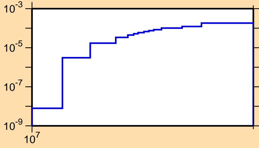
\sigma vs. E for ^{120}\text{La}(n,2n)
