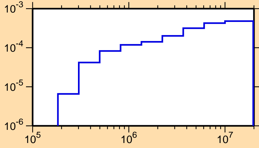
\sigma vs. E for ^{120}\text{La}(n,n_1)
