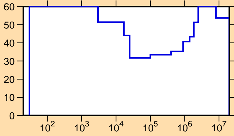
\Delta\sigma/\sigma vs. E for ^{120}\text{La}(n,p)
