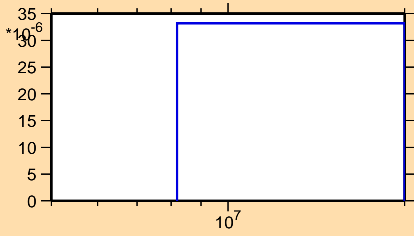
\sigma vs. E for ^{120}\text{La}(n,pt)
