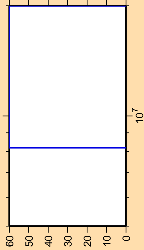
\Delta\sigma/\sigma vs. E for ^{120}\text{La}(n,pt)
