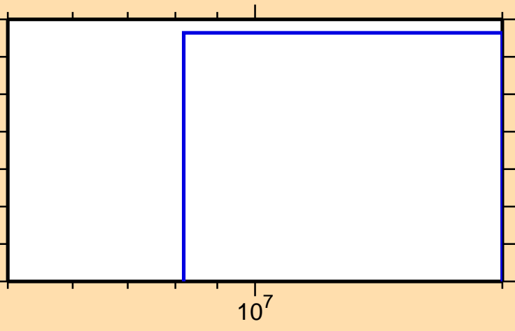
\sigma vs. E for ^{120}\text{La}(n,pt)
