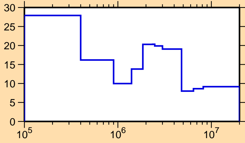
\Delta\sigma/\sigma vs. E for ^{120}\text{La}(n, el.)
