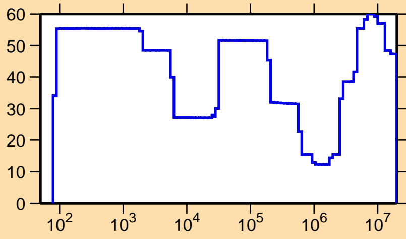
\Delta\sigma/\sigma vs. E for ^{121}\text{La}(n,p)
