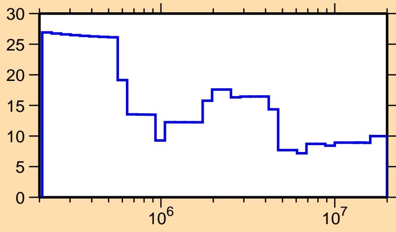
\Delta\sigma/\sigma vs. E for ^{121}\text{La}(n, el.)
