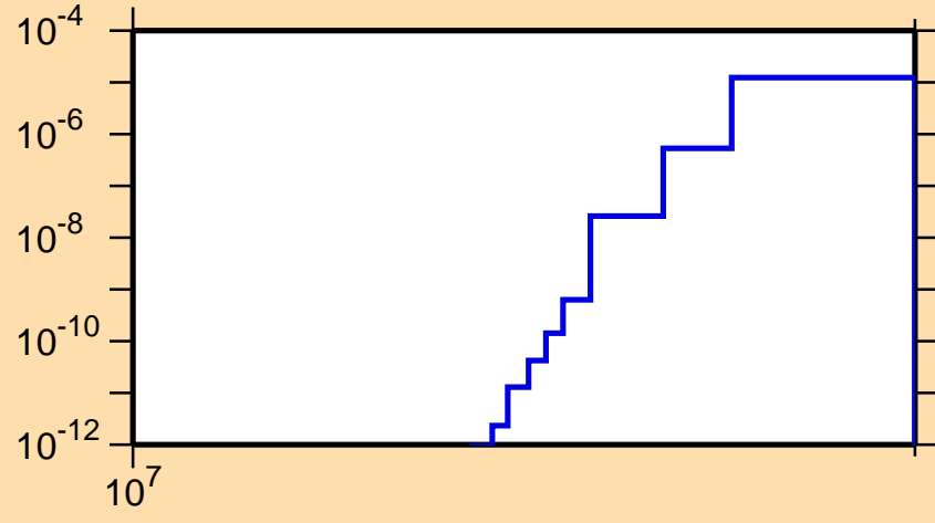
\sigma vs. E for ^{121}\text{La}(n,pt)
