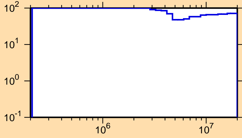
\Delta\sigma/\sigma vs. E for ^{121}\text{La}(n,n\text{cont.})
