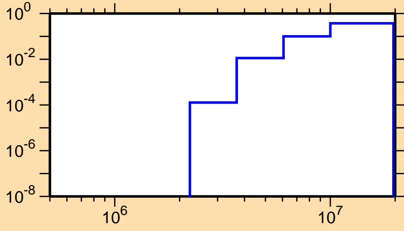
\sigma vs. E for ^{121}\text{La}(n,np)
