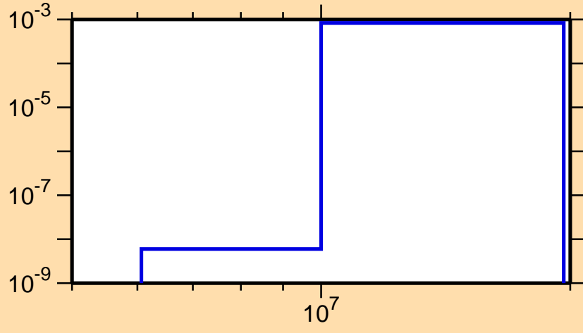
\sigma vs. E for ^{121}\text{La}(n,\text{pd})
