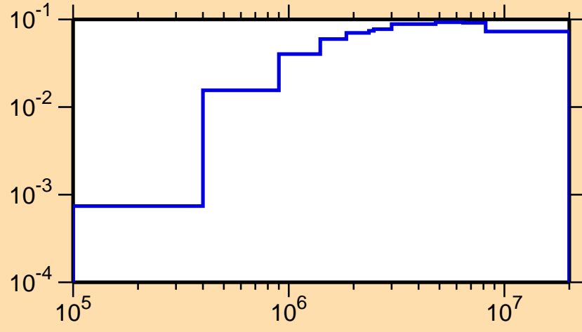
\sigma vs. E for ^{121}\text{La}(n,\text{inel.})
