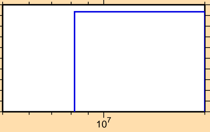
\sigma vs. E for ^{121}\text{La}(n,2np)
