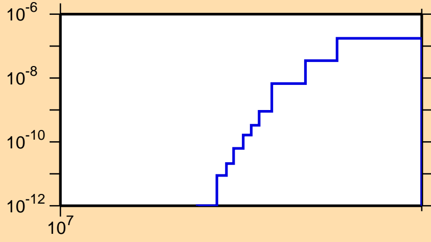
\sigma vs. E for ^{122}\text{La}(n,2n\alpha)
