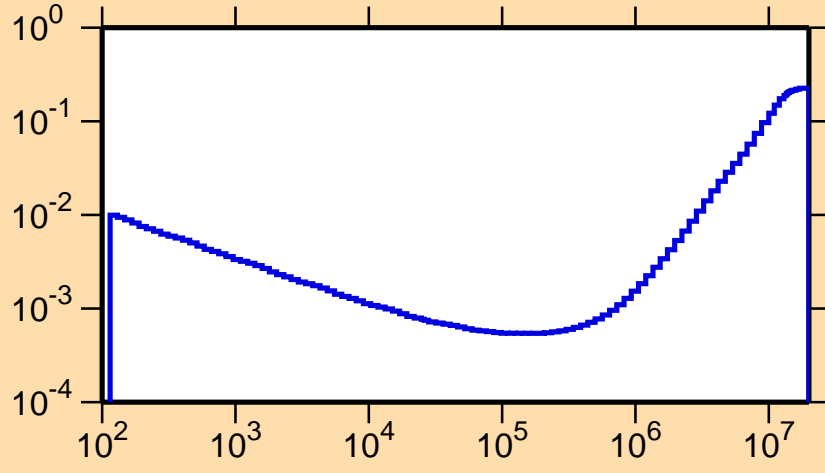
\sigma vs. E for ^{122}\text{La}(n,p\alpha)
