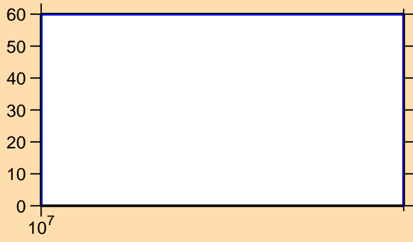
\Delta\sigma/\sigma vs. E for ^{122}\text{La}(n,2n)
