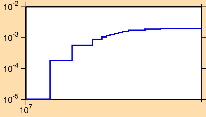
\sigma vs. E for ^{122}\text{La}(n,2n)
