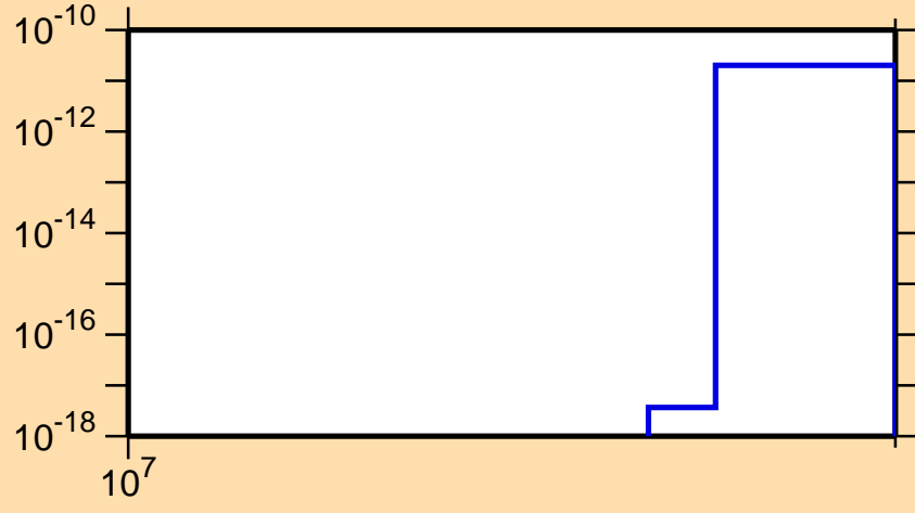
\sigma vs. E for ^{122}\text{La}(n,nt)
