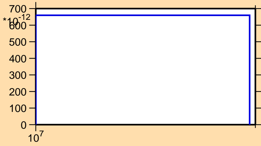
\sigma vs. E for ^{122}\text{La} (mt 34)
