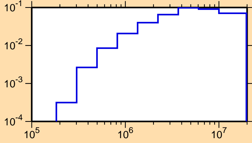
\sigma vs. E for ^{122}\text{La}(n,\text{inel.})
