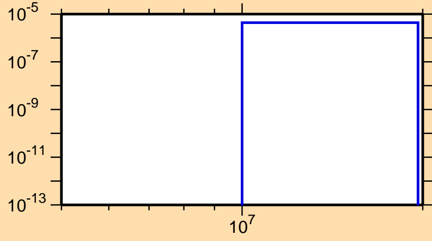
\sigma vs. E for ^{122}\text{La}(n,\text{pt})
