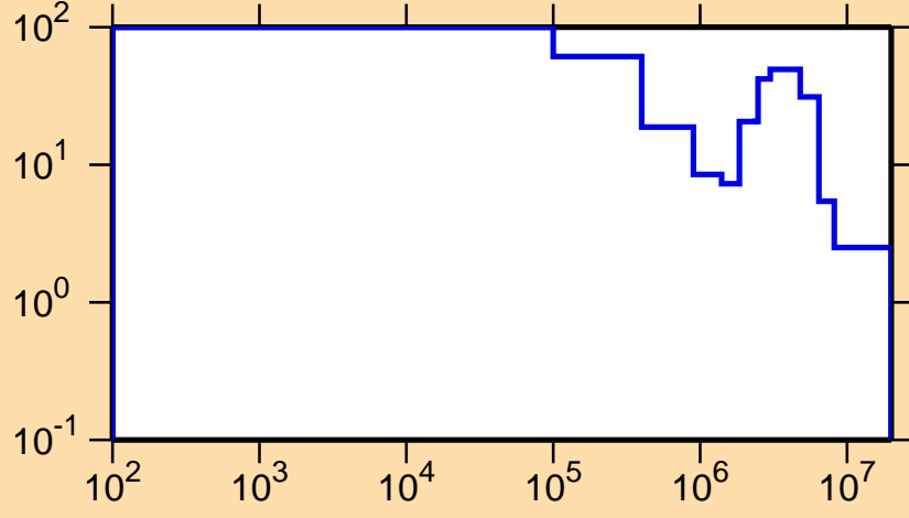
\Delta\sigma/\sigma vs. E for ^{122}\text{La}(n,el.)
