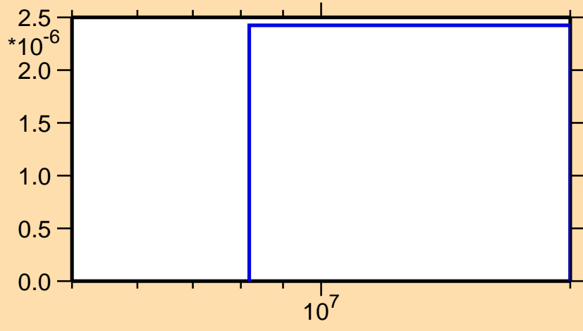
\sigma vs. E for ^{122}\text{La}(n,\text{nd})
