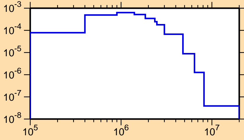
\sigma vs. E for ^{122}\text{La}(n,n_1)
