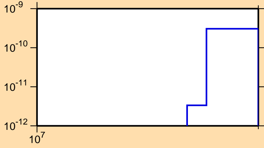
\sigma vs. E for ^{123}\text{La} (mt 34)
