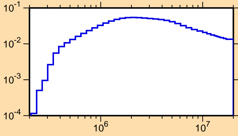
\sigma vs. E for ^{123}\text{La}(n,n_1)
