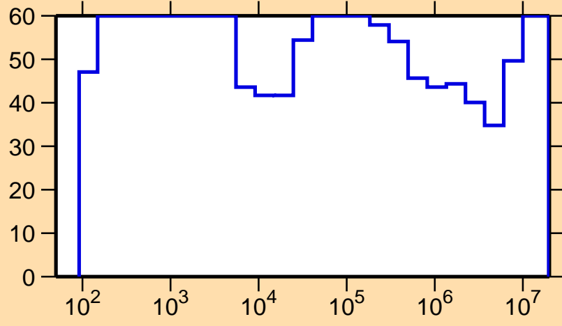
\Delta\sigma/\sigma vs. E for ^{123}\text{La}(n,p)
