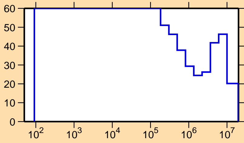
\Delta\sigma/\sigma vs. E for ^{123}\text{La}(n,el.)
