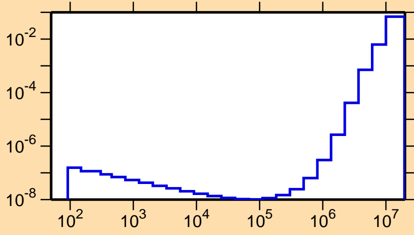
\sigma vs. E for ^{123}\text{La}(n,p\alpha)
