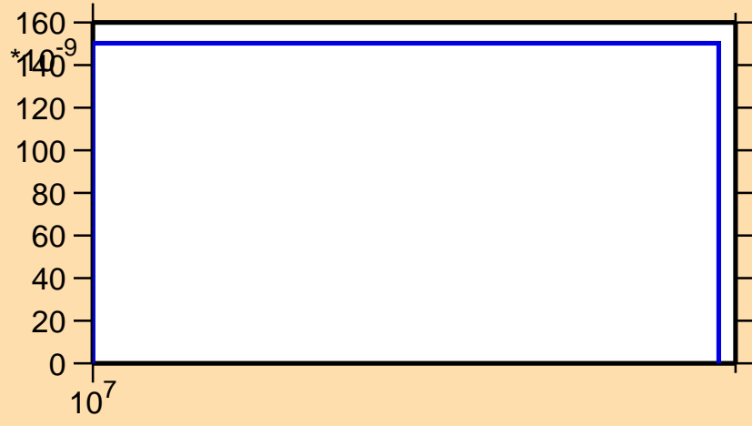
\sigma vs. E for ^{123}\text{La}(n,\text{nd})
