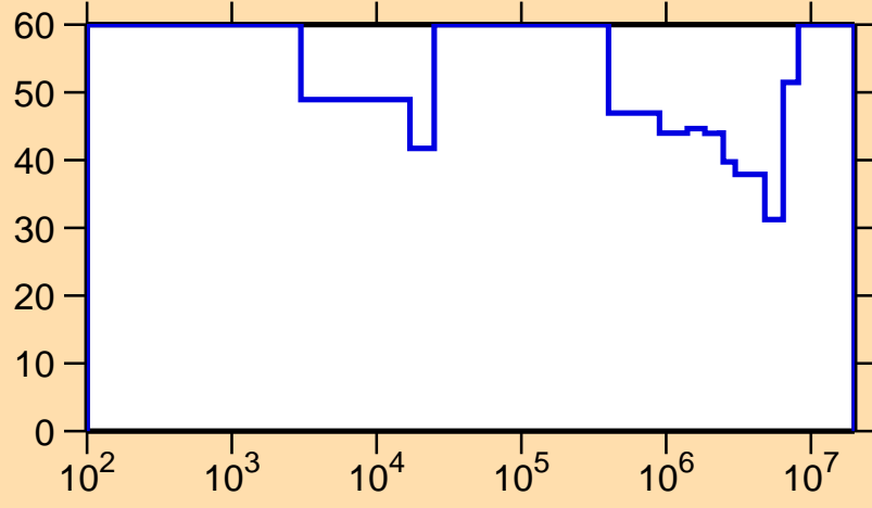
\Delta\sigma/\sigma vs. E for ^{123}\text{La}(n,p)
