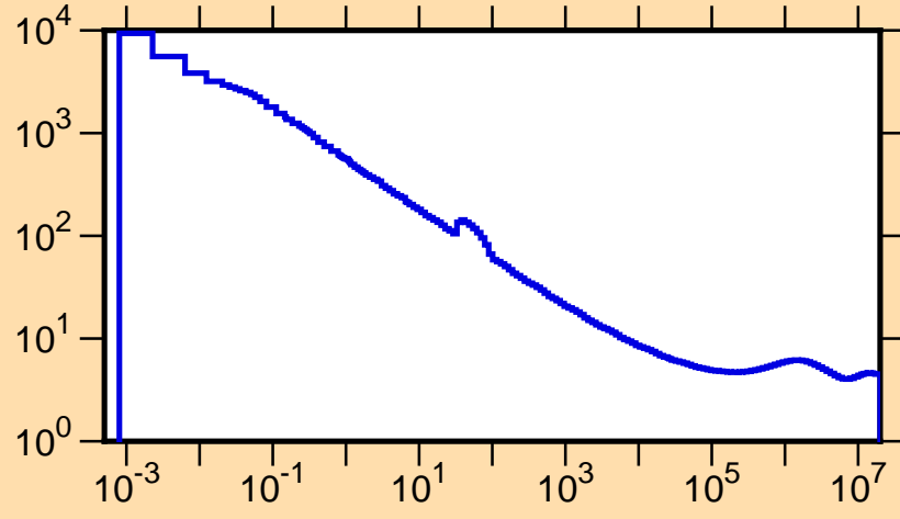
\sigma vs. E for ^{124}\text{La}(n,\text{tot.})
