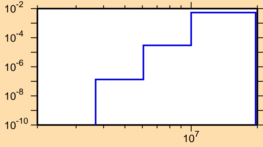
\sigma vs. E for ^{124}\text{La}(n,n\alpha)
