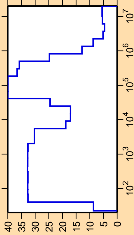
\Delta\sigma/\sigma vs. E for ^{124}\text{La}(n,\text{nonel.})
