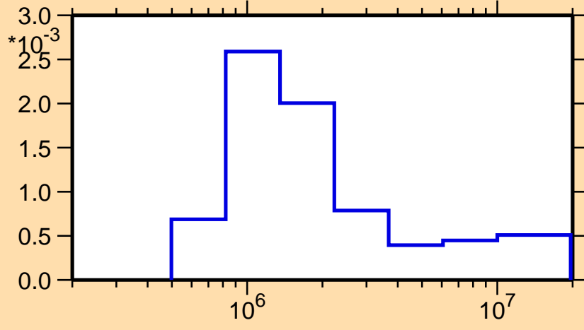
\sigma vs. E for ^{124}\text{La}(n,n_4)
