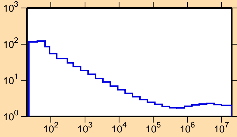
\sigma vs. E for ^{124}\text{La}(n,\text{nonel.})
