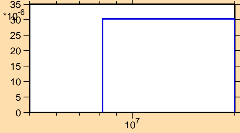
\sigma vs. E for ^{124}\text{La}(n,\text{pd})
