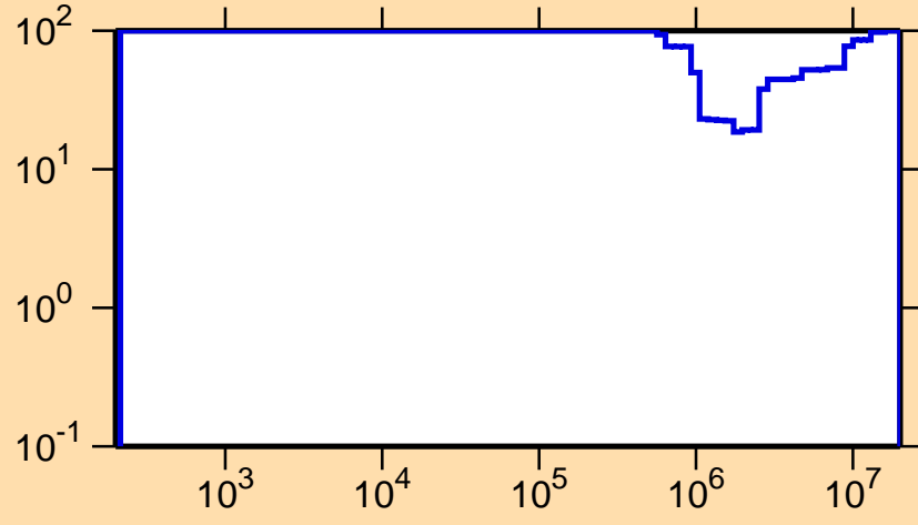
\Delta\sigma/\sigma vs. E for ^{125}\text{La}(n,p)
