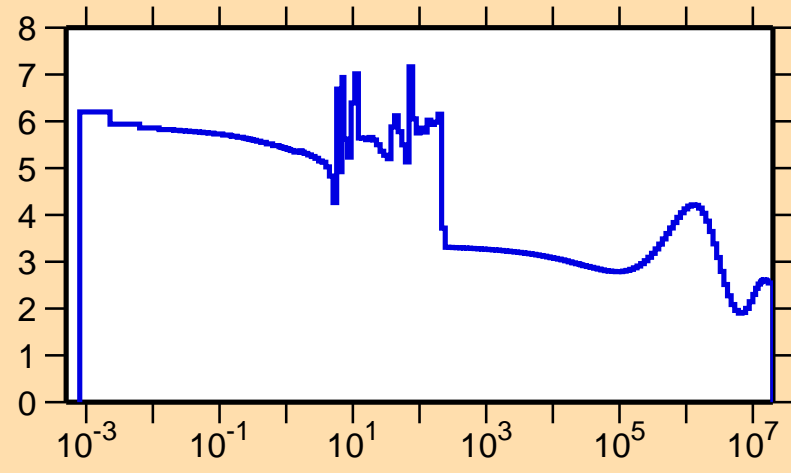
\sigma vs. E for ^{125}\text{La}(n,\text{el.})
