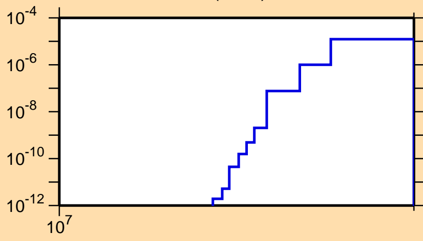
\sigma vs. E for ^{125}\text{La}(n,\text{nd})
