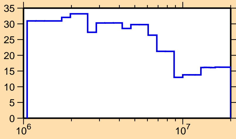
\Delta\sigma/\sigma vs. E for ^{125}\text{La}(n,\text{el.})
