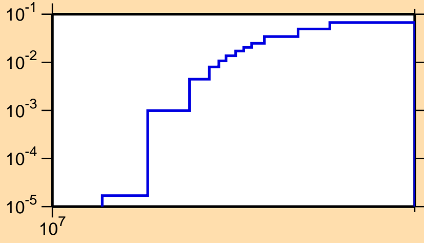
\sigma vs. E for ^{125}\text{La}(n,2n)
