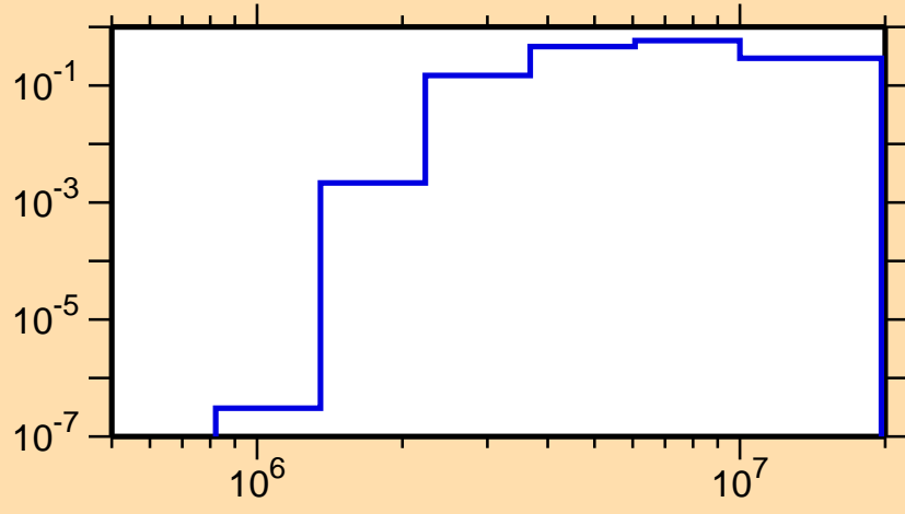
\sigma vs. E for ^{125}\text{La}(n,n\text{cont.})
