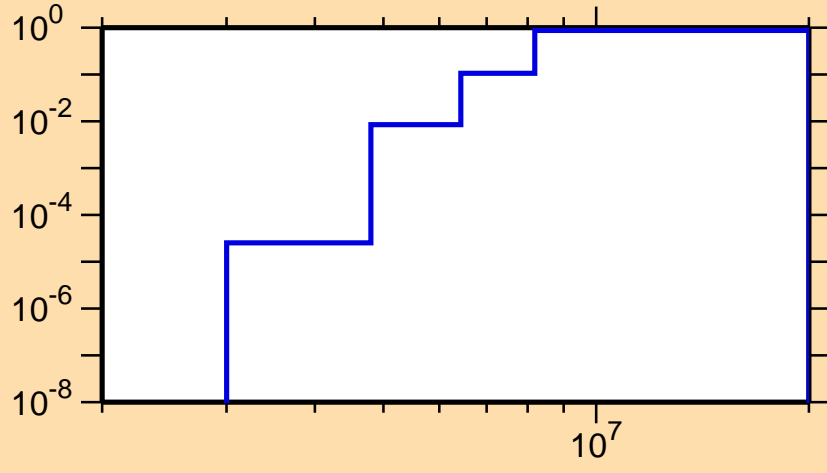
\sigma vs. E for ^{125}\text{La}(n,np)
