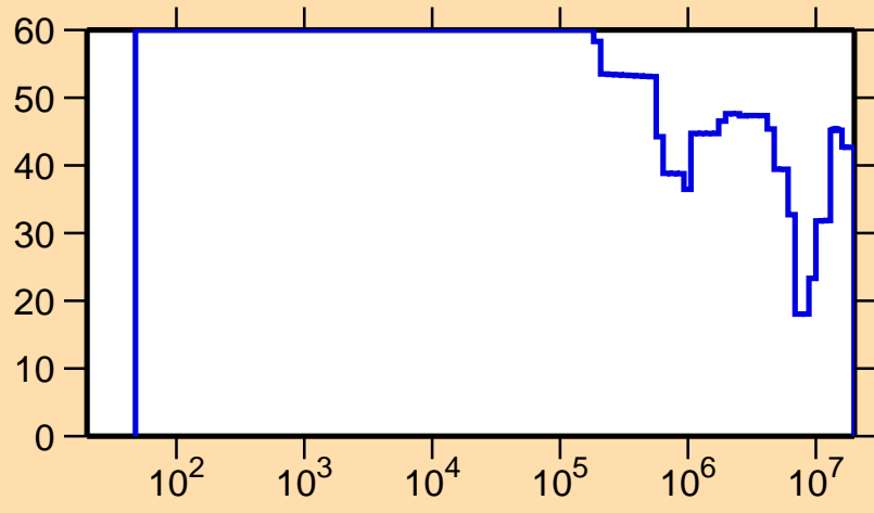
\Delta\sigma/\sigma vs. E for ^{126}\text{La}(n,p)
