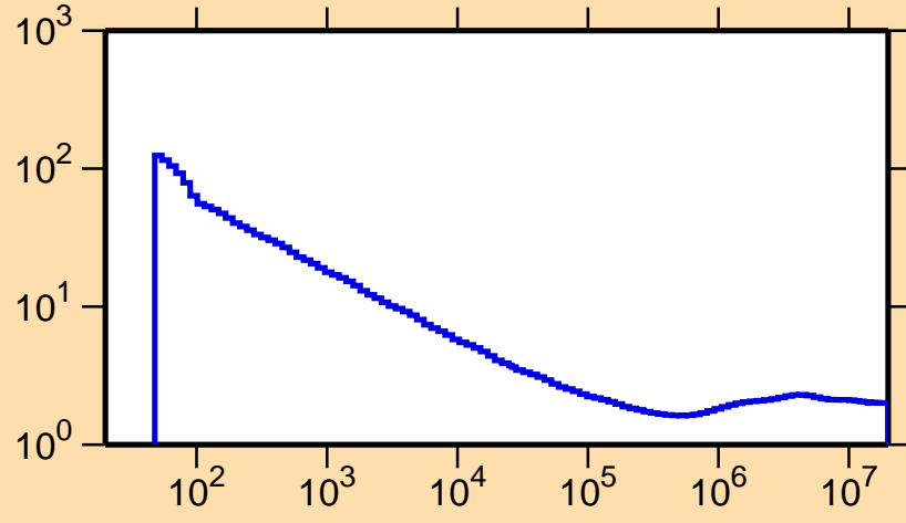
\sigma vs. E for ^{126}\text{La}(n,\text{nonel.})
