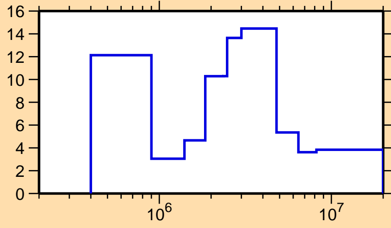
\Delta\sigma/\sigma vs. E for ^{126}\text{La}(n, el.)
