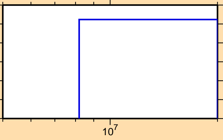
\sigma vs. E for ^{126}\text{La}(n,\text{nd})
