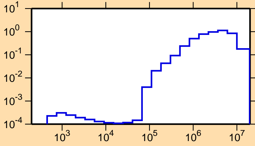
\sigma vs. E for ^{126}\text{La}(n,\text{inel.})
