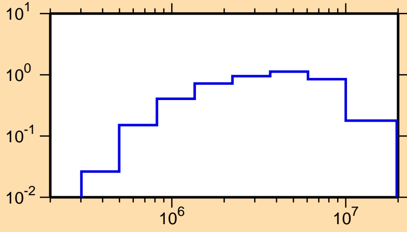
\sigma vs. E for ^{126}\text{La}(n,n\text{cont.})
