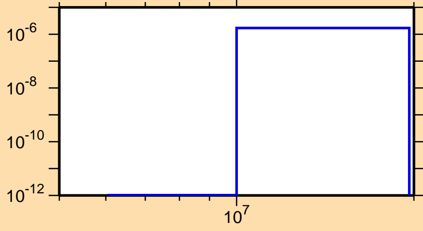
\sigma vs. E for ^{126}\text{La}(\text{mt117})
