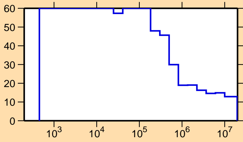
\Delta\sigma/\sigma vs. E for ^{126}\text{La}(n,\text{nonel.})
