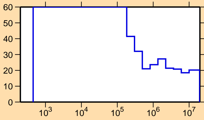
\Delta\sigma/\sigma vs. E for ^{126}\text{La}(n,\text{tot.})
