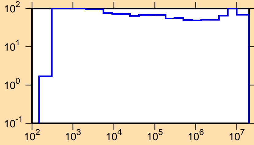
\Delta\sigma/\sigma vs. E for ^{126}\text{La}(n,p)
