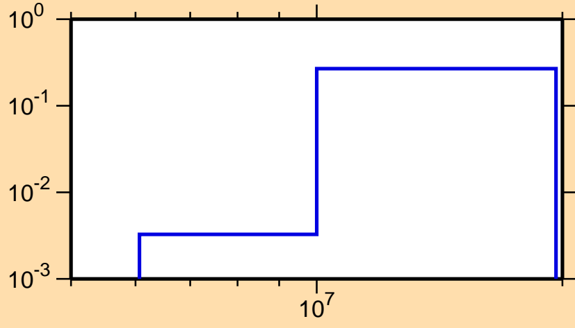
\sigma vs. E for ^{126}\text{La}(n,2n)
