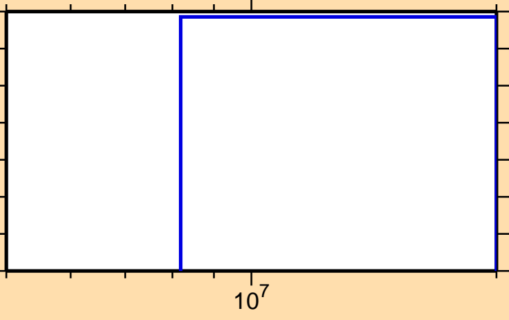
\sigma vs. E for ^{126}\text{La}(\text{mt117})
