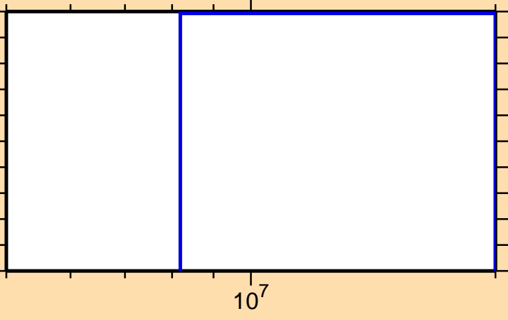
\sigma vs. E for ^{126}\text{La}(n,nt)
