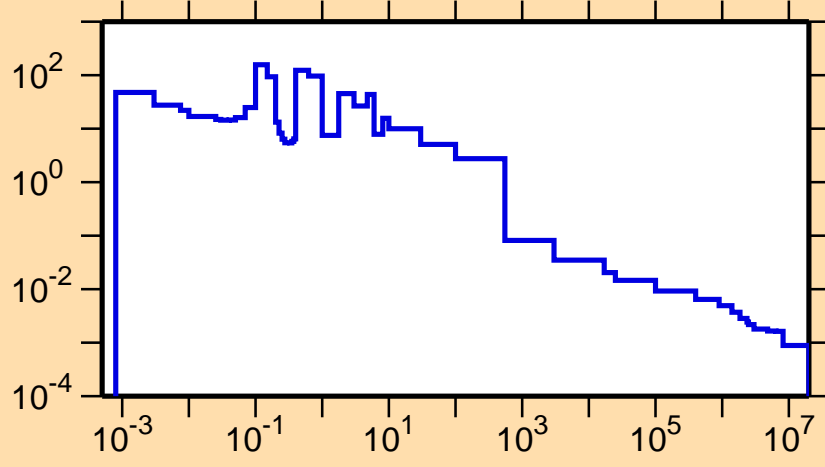
\sigma vs. E for ^{126}\text{La}(n,\gamma)
