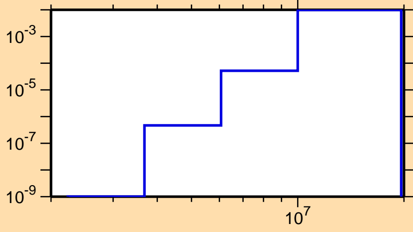
\sigma vs. E for ^{127}\text{La}(n,d)
