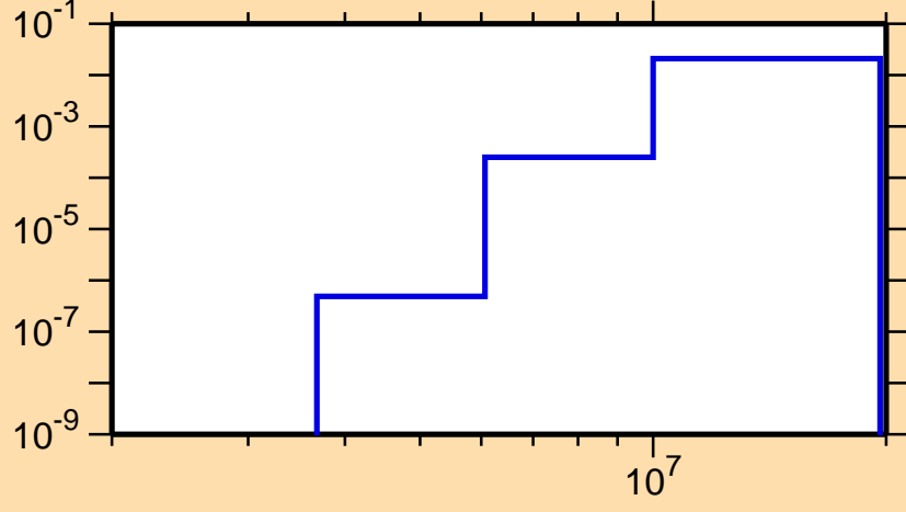
\sigma vs. E for ^{127}\text{La}(n,n\alpha)
