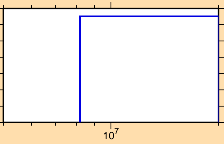
\sigma vs. E for ^{127}\text{La}(n,2np)
