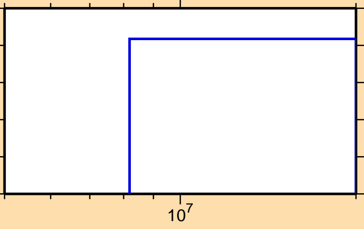
\sigma vs. E for ^{127}\text{La}(n,pd)
