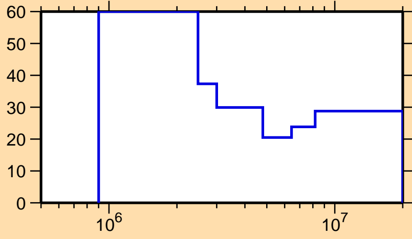
\Delta\sigma/\sigma vs. E for ^{127}\text{La}(n,n\text{cont.})
