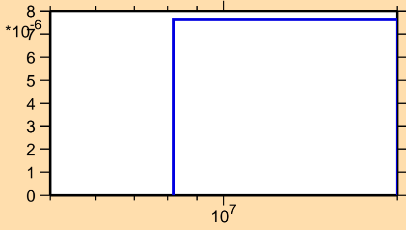
\sigma vs. E for ^{127}\text{La} (mt 45)
