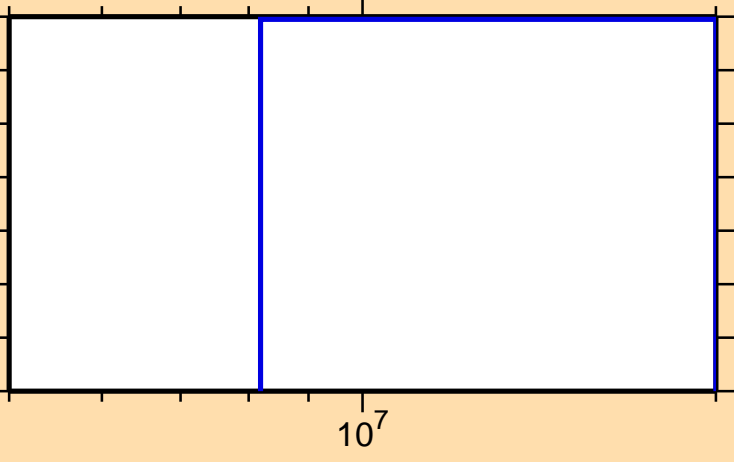
\sigma vs. E for ^{127}\text{La}(\text{mt117})
