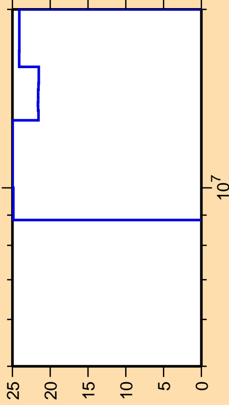
\Delta\sigma/\sigma vs. E for ^{128}\text{La}(n,2n)
