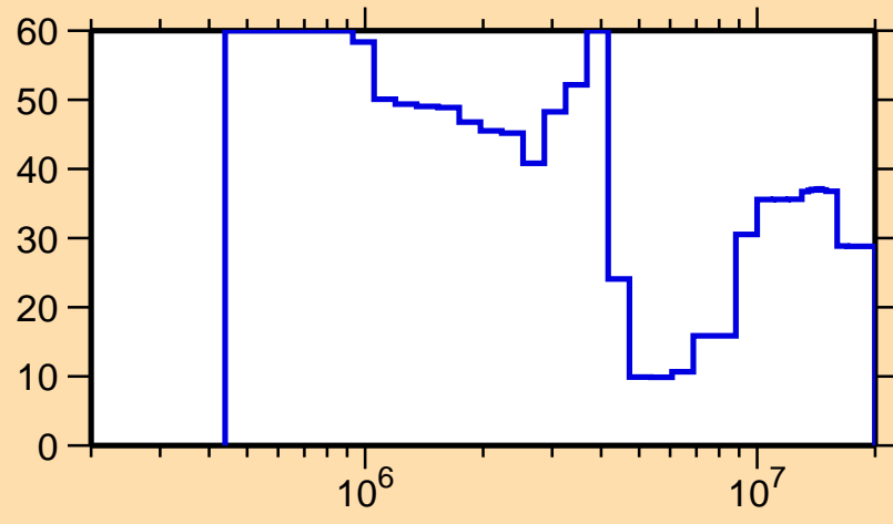
\Delta\sigma/\sigma vs. E for ^{128}\text{La}(n,n\text{cont.})
