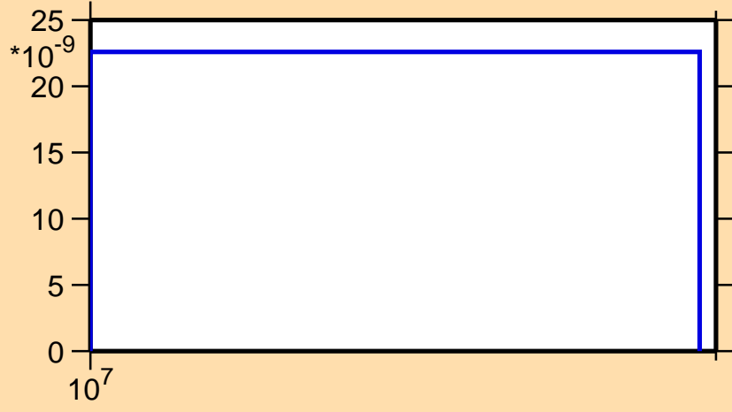
\sigma vs. E for ^{128}\text{La}(n,\text{pd})
