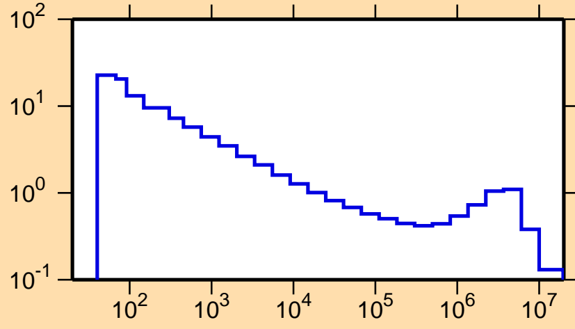
\sigma vs. E for ^{128}\text{La}(n,p)
