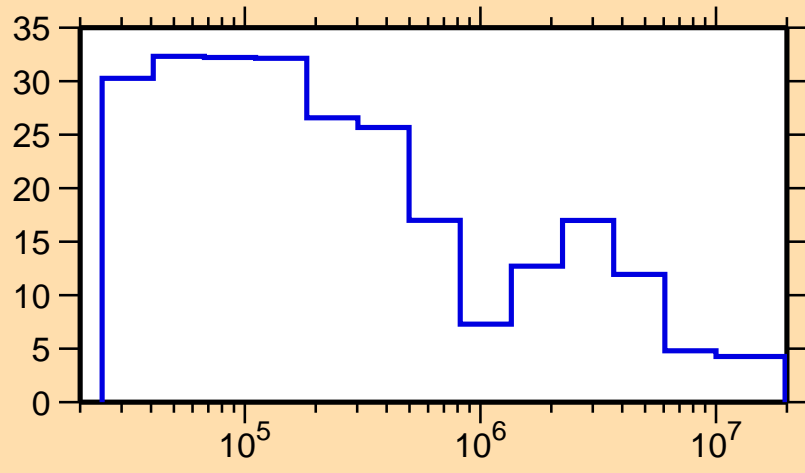
\Delta\sigma/\sigma vs. E for ^{128}\text{La}(n,\text{el.})
