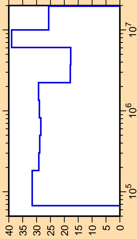
\Delta\sigma/\sigma vs. E for ^{128}\text{La}(n,n_2)
