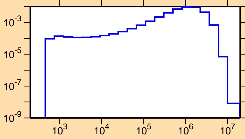
\sigma vs. E for ^{128}\text{La}(n,n_2)
