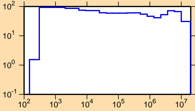
\Delta\sigma/\sigma vs. E for ^{128}\text{La}(n,p)
