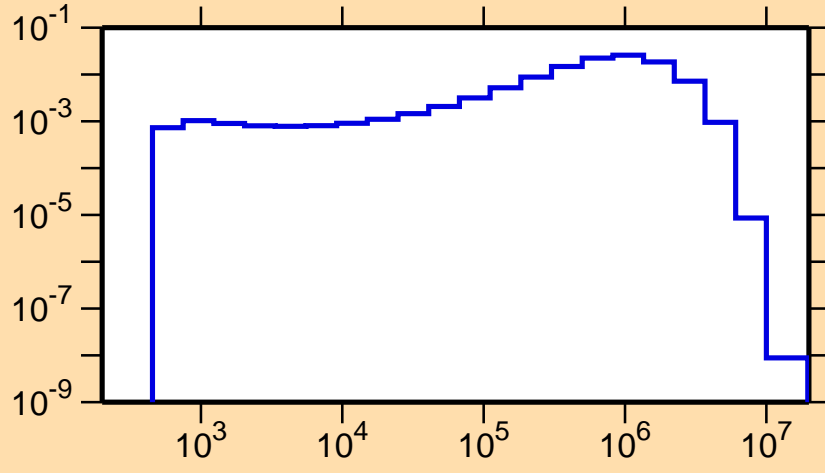
\sigma vs. E for ^{128}\text{La}(n,n_1)
