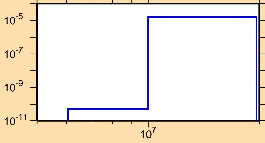
\sigma vs. E for ^{128}\text{La}(n,\text{He3})
