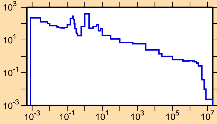
\sigma vs. E for ^{128}\text{La}(n,\gamma)
