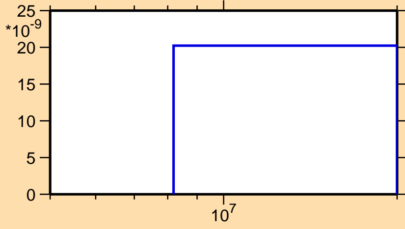
\sigma vs. E for ^{128}\text{La}(\text{mt117})
