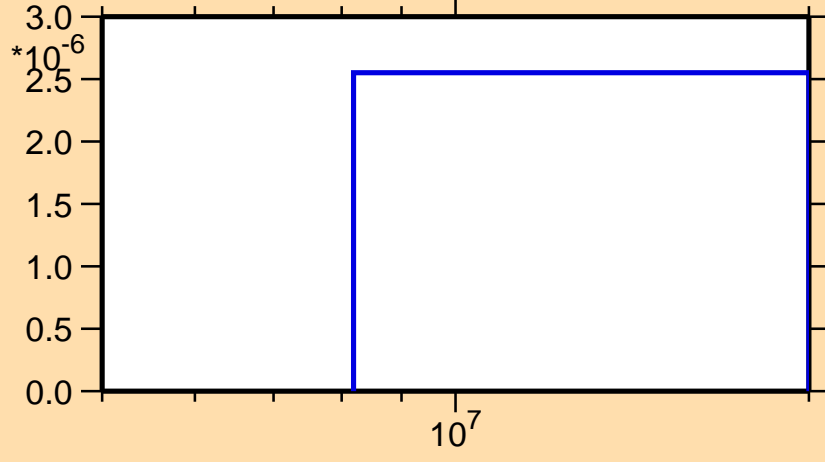
\sigma vs. E for ^{128}\text{La}(n,2n\alpha)
