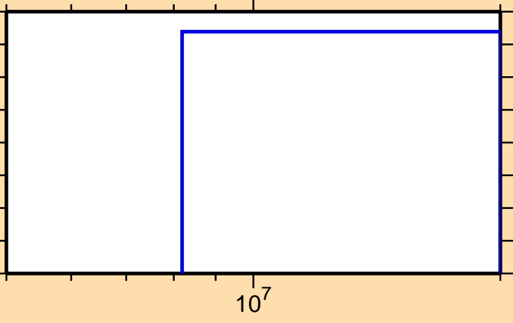
\sigma vs. E for ^{128}\text{La}(n,\text{nd})
