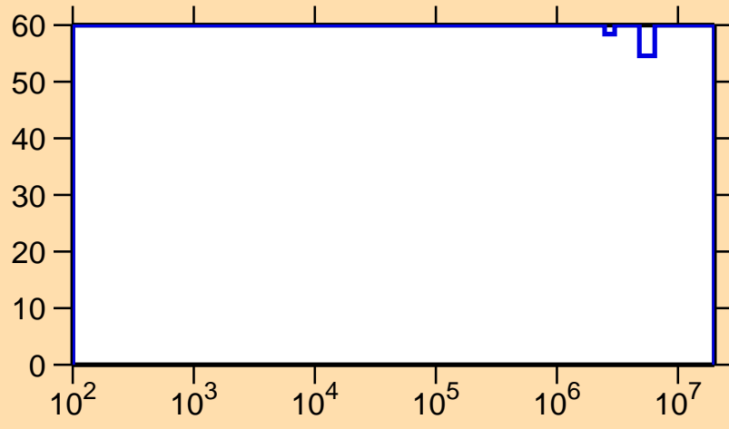
\Delta\sigma/\sigma vs. E for ^{128}\text{La}(n,n_1)
