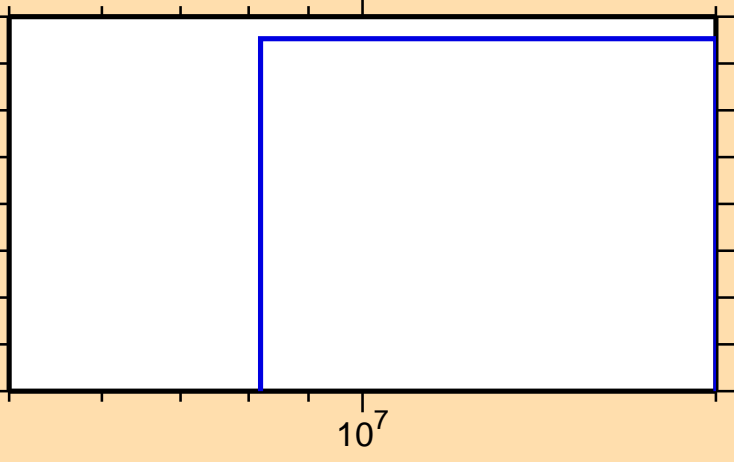
\sigma vs. E for ^{128}\text{La}(n,pd)
