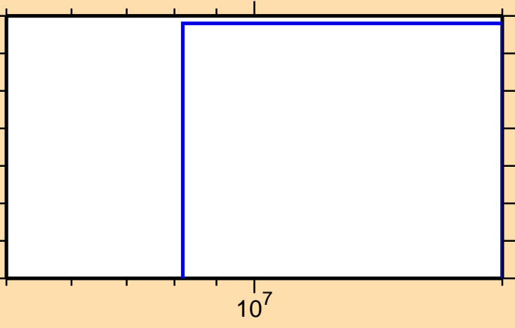
\sigma vs. E for ^{128}\text{La} (mt 45)
