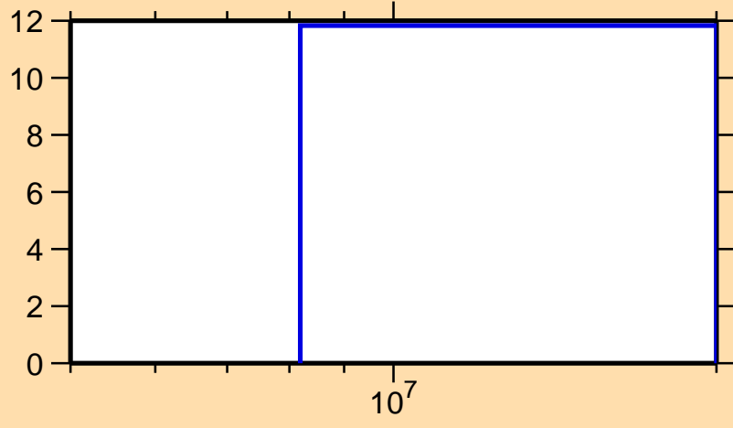
\Delta\sigma/\sigma vs. E for ^{128}\text{La}(n,\text{tot.})
