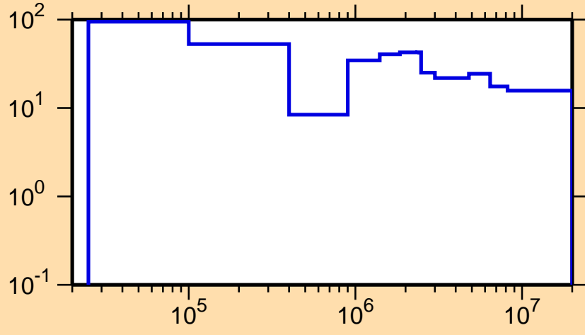
\Delta\sigma/\sigma vs. E for ^{128}\text{La}(n, el.)
