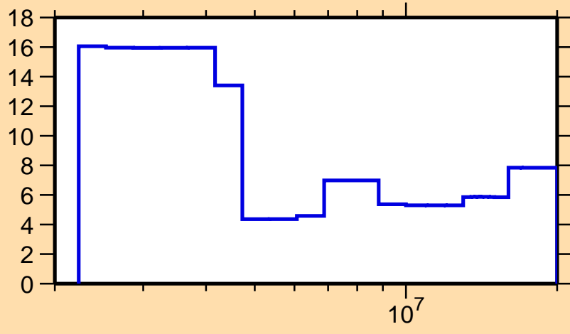
\Delta\sigma/\sigma vs. E for ^{129}\text{La}(n, el.)
