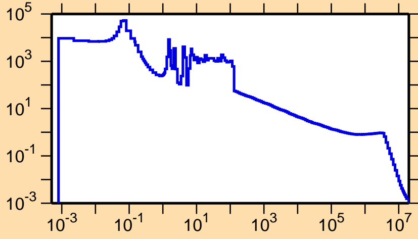
\sigma vs. E for ^{129}\text{La}(n,\gamma)
