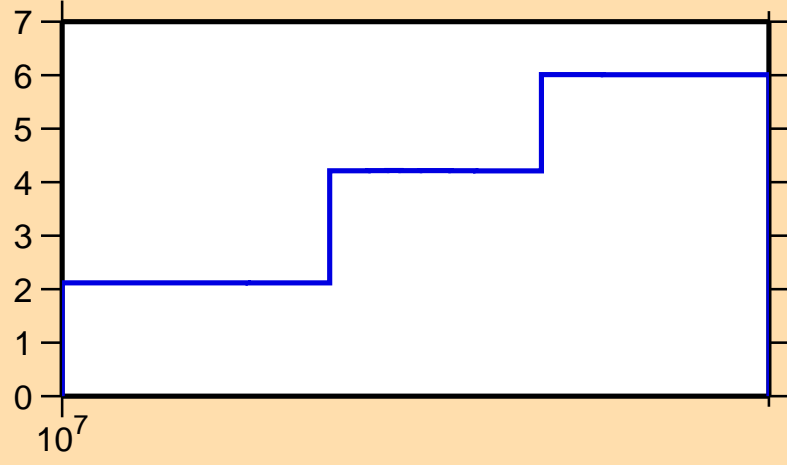
\Delta\sigma/\sigma vs. E for ^{129}\text{La}(n,\text{tot.})
