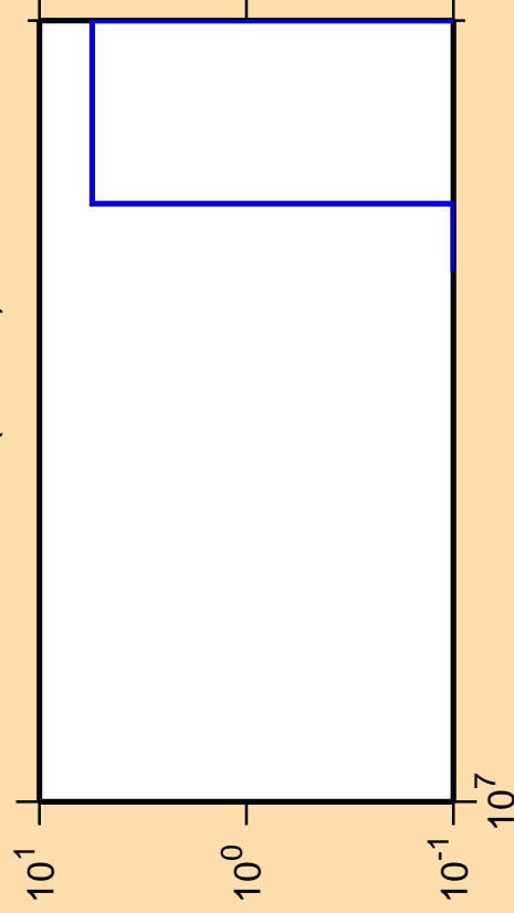
\Delta\sigma/\sigma vs. E for ^{129}\text{La} (mt 34)
