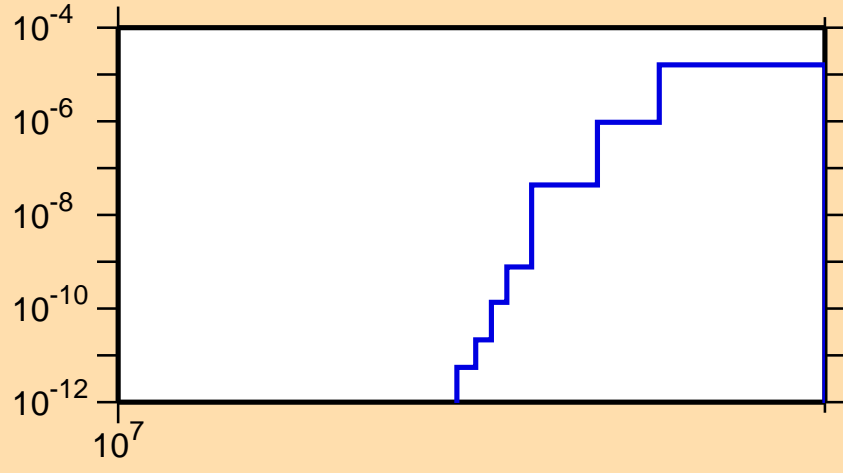
\sigma vs. E for ^{129}\text{La}(n,\text{nd})
