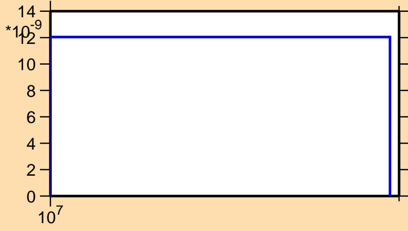
\sigma vs. E for ^{129}\text{La}(n,\text{pd})
