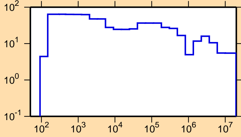
\Delta\sigma/\sigma vs. E for ^{129}\text{La}(n,el.)
