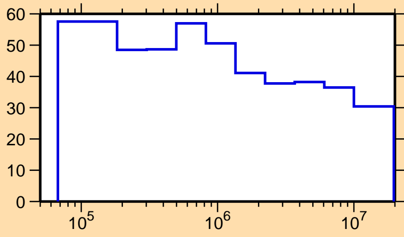
\Delta\sigma/\sigma vs. E for ^{129}\text{La}(n,n_1)
