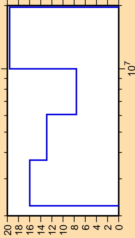
\Delta\sigma/\sigma vs. E for ^{129}\text{La}(n,n\text{cont.})
