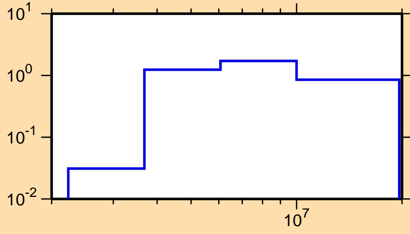
\sigma vs. E for ^{129}\text{La}(n,n\text{cont.})
