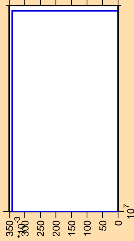
\Delta\sigma/\sigma vs. E for ^{129}\text{La}(n,\text{pt})
