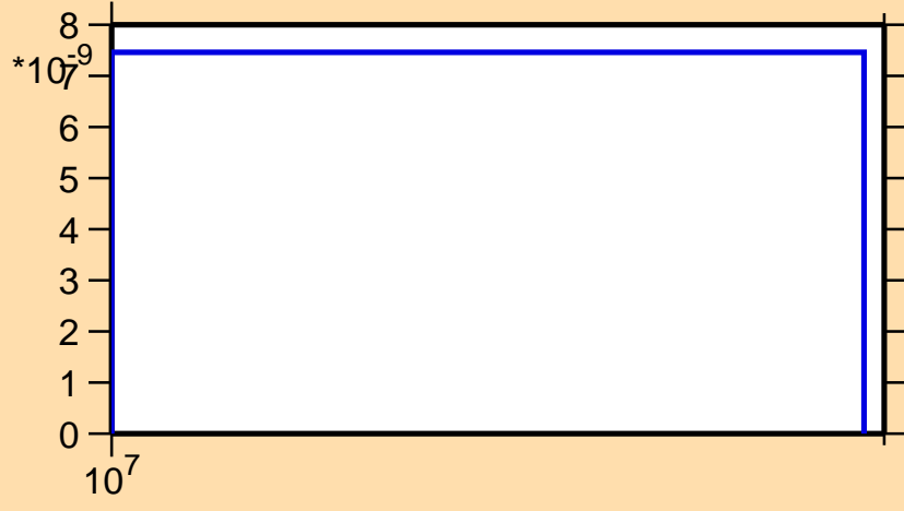
\sigma vs. E for ^{129}\text{La}(n,2n\alpha)
