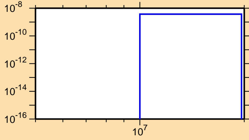
\sigma vs. E for ^{129}\text{La}(\text{mt117})
