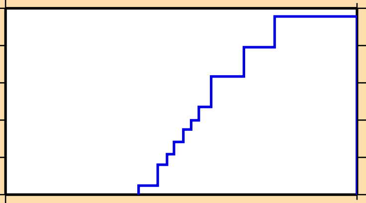
\sigma vs. E for ^{130}\text{La} (mt 45)
