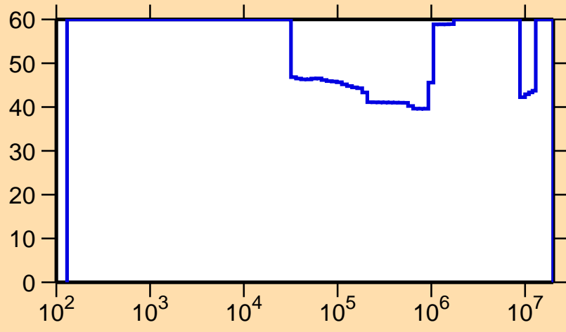
\Delta\sigma/\sigma vs. E for ^{130}\text{La}(n,\gamma)
