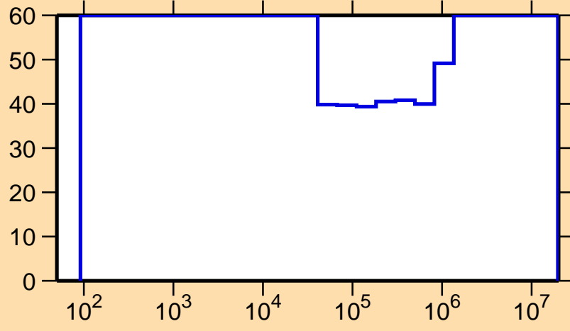
\Delta\sigma/\sigma vs. E for ^{130}\text{La}(n,\gamma)
