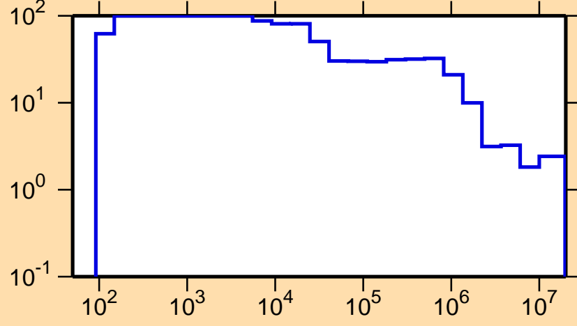
\Delta\sigma/\sigma vs. E for ^{130}\text{La}(n,\text{nonel.})
