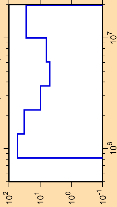
\Delta\sigma/\sigma vs. E for ^{130}\text{La}(n,\text{ncont.})
