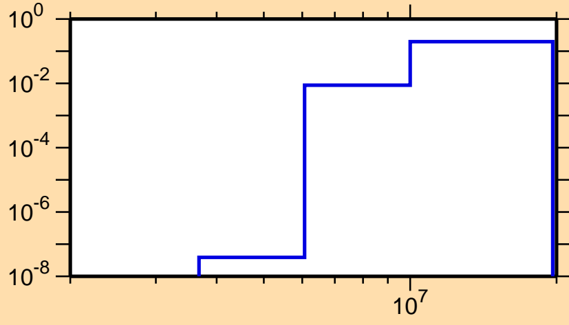
\sigma vs. E for ^{130}\text{La}(n,np)
