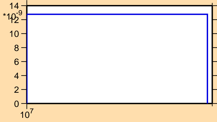
\sigma vs. E for ^{130}\text{La} (mt 45)
