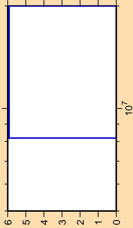
\Delta\sigma/\sigma vs. E for ^{130}\text{La}(n,2n)
