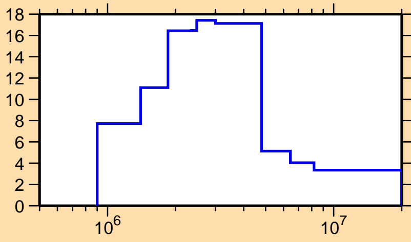
\Delta\sigma/\sigma vs. E for ^{130}\text{La}(n, el.)
