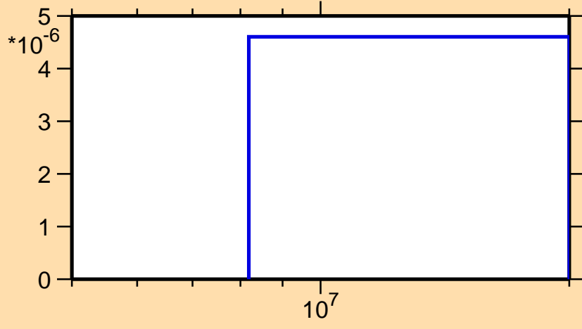
\sigma vs. E for ^{130}\text{La}(n,\text{nd})
