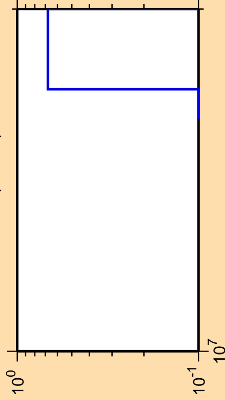
\Delta\sigma/\sigma vs. E for ^{131}\text{La} (mt 34)
