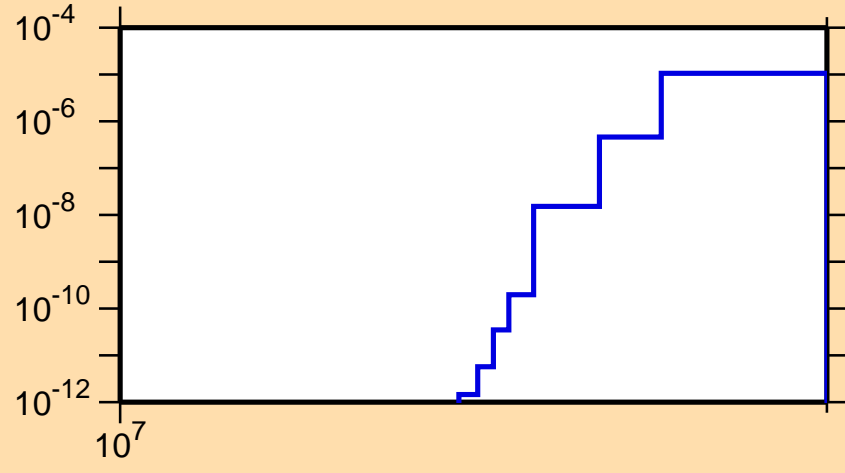
\sigma vs. E for ^{131}\text{La}(n,\text{nd})
