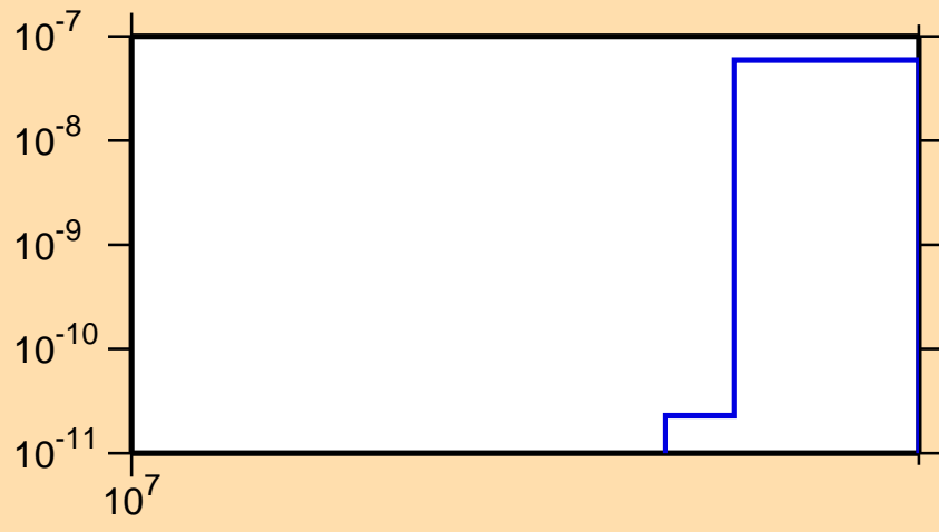
\sigma vs. E for ^{131}\text{La}(n,nt)
