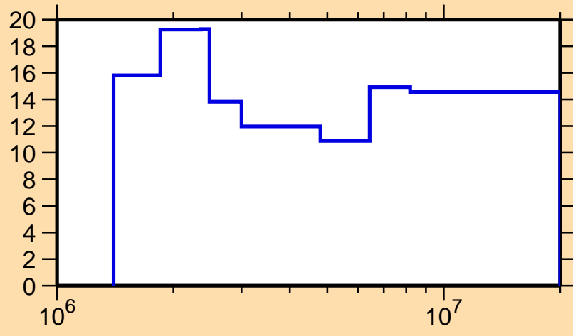
\Delta\sigma/\sigma vs. E for ^{131}\text{La}(n, el.)
