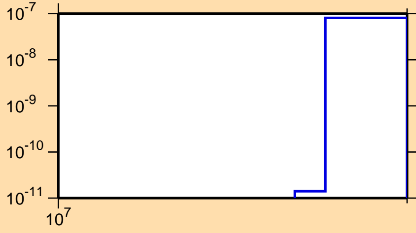
\sigma vs. E for ^{132}\text{La}(n,nt)
