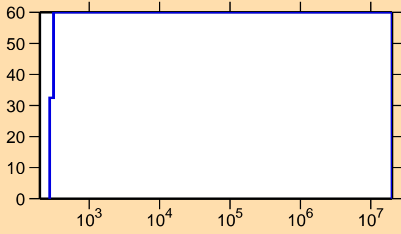
\Delta\sigma/\sigma vs. E for ^{132}\text{La}(n,\gamma)
