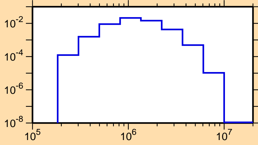
\sigma vs. E for ^{132}\text{La}(n,n_4)
