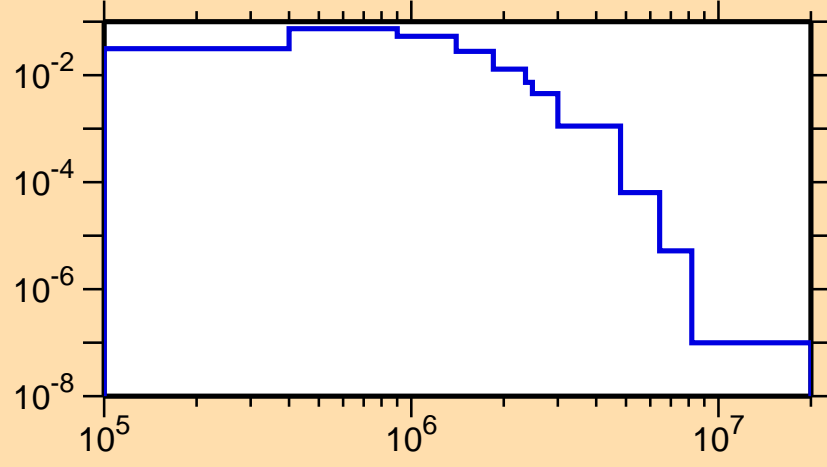
\sigma vs. E for ^{132}\text{La}(n,n_3)
