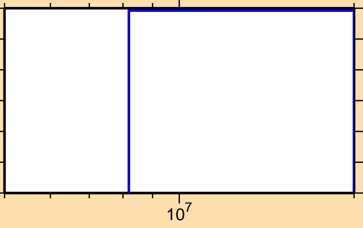
\sigma vs. E for ^{132}\text{La}(n,2np)
