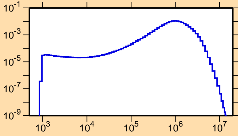
\sigma vs. E for ^{132}\text{La}(n,n_1)
