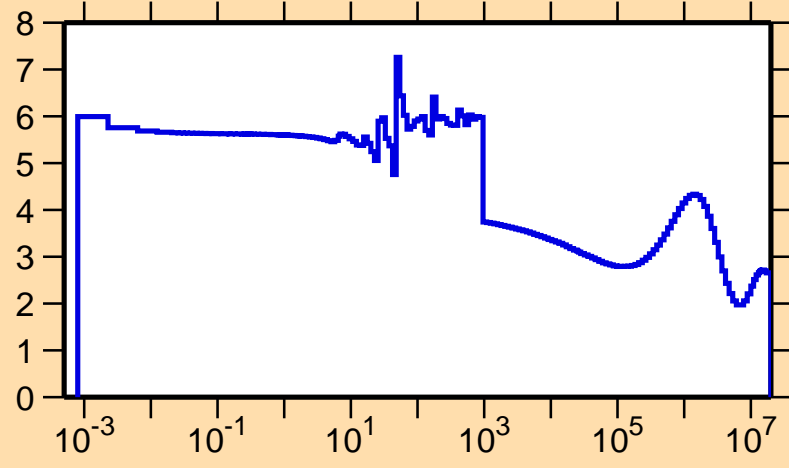
\sigma vs. E for ^{132}\text{La}(n,\text{el.})
