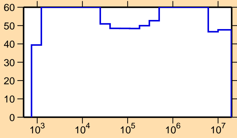
\Delta\sigma/\sigma vs. E for ^{132}\text{La}(n,p)
