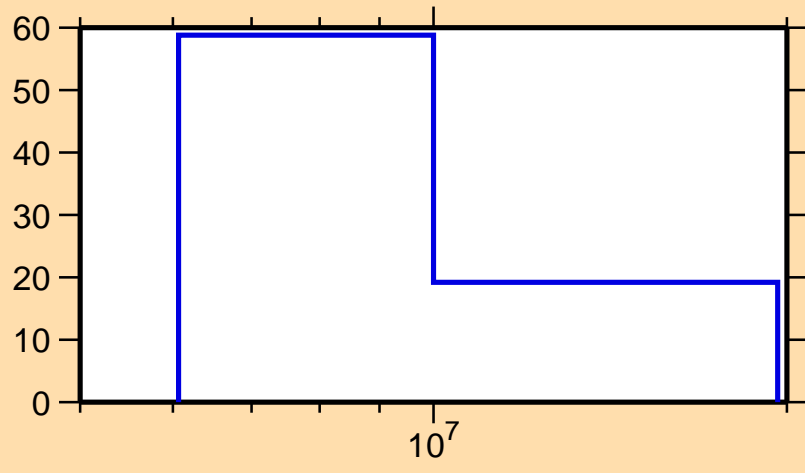
\Delta\sigma/\sigma vs. E for ^{132}\text{La}(n,2n)
