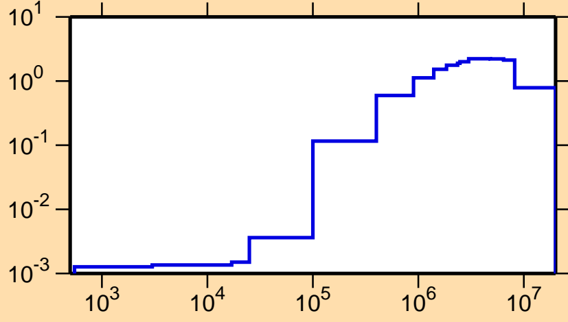
\sigma vs. E for ^{132}\text{La}(n,\text{inel.})
