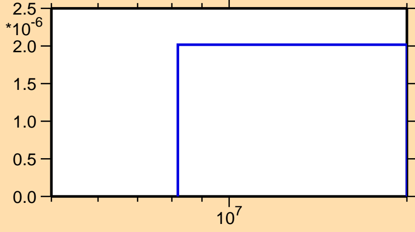
\sigma vs. E for ^{132}\text{La}(n,\text{nd})
