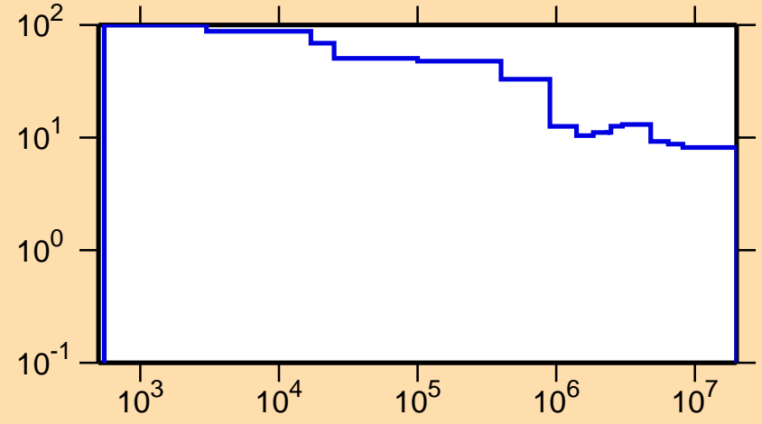
\Delta\sigma/\sigma vs. E for ^{132}\text{La}(n,\text{nonel.})
