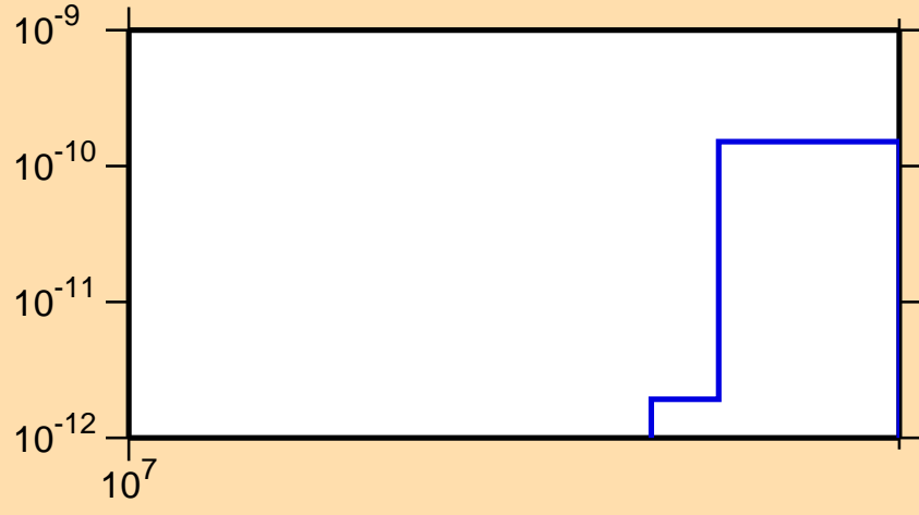
\sigma vs. E for ^{133}\text{La}(n,pd)
