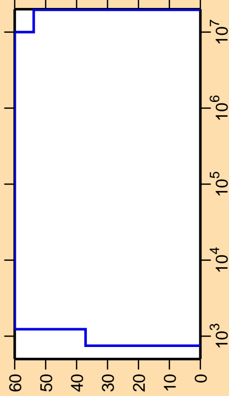
\Delta\sigma/\sigma vs. E for ^{133}\text{La}(n,\alpha)
