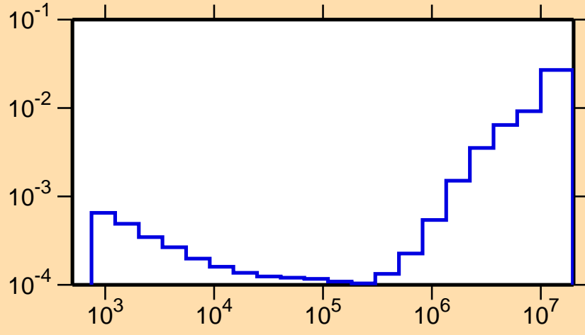
\sigma vs. E for ^{133}\text{La}(n,p)
