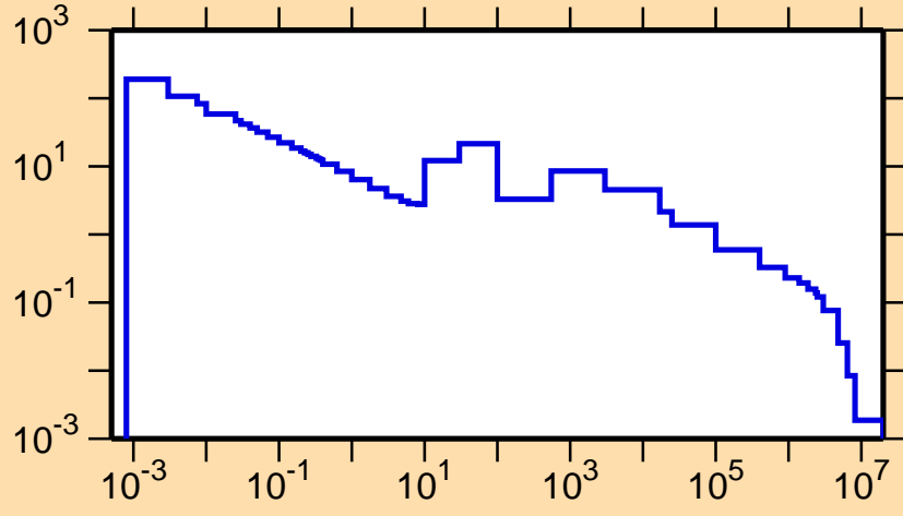
\sigma vs. E for ^{133}\text{La}(n,\gamma)
