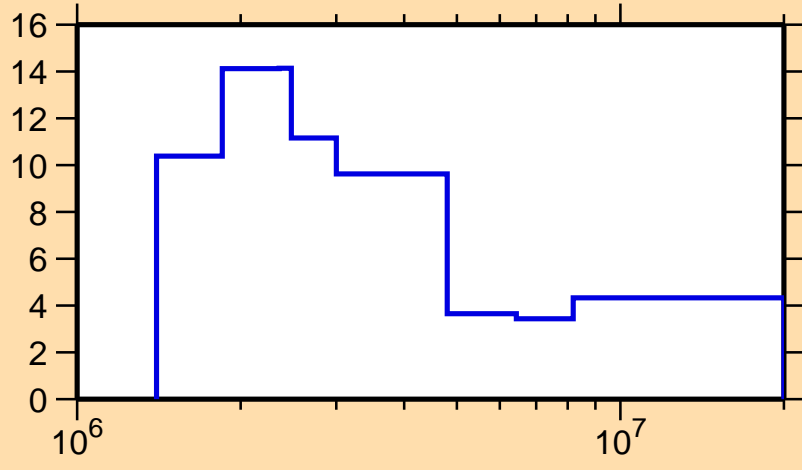
\Delta\sigma/\sigma vs. E for ^{133}\text{La}(n,\text{tot.})
