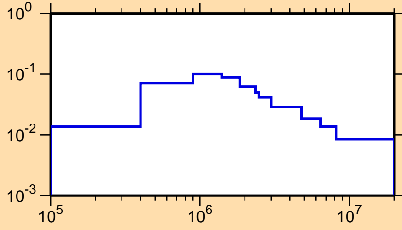
\sigma vs. E for ^{133}\text{La}(n,n_4)
