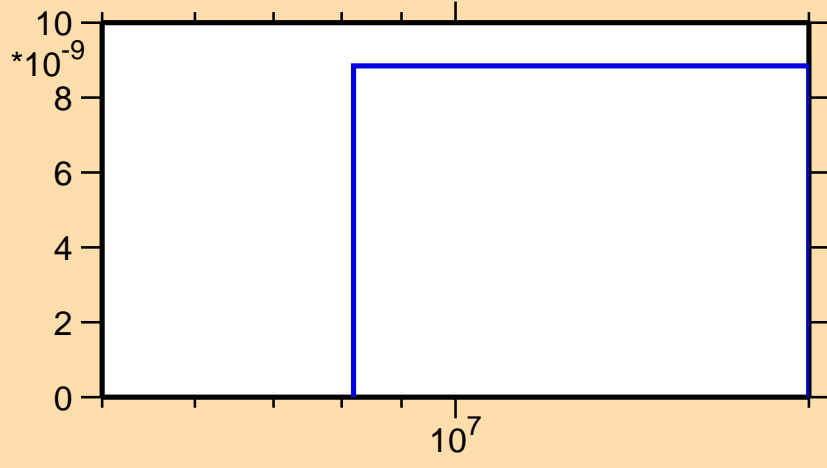
\sigma vs. E for ^{133}\text{La}(n,\text{He3})
