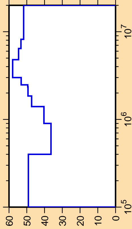
\Delta\sigma/\sigma vs. E for ^{133}\text{La}(n,n_4)
