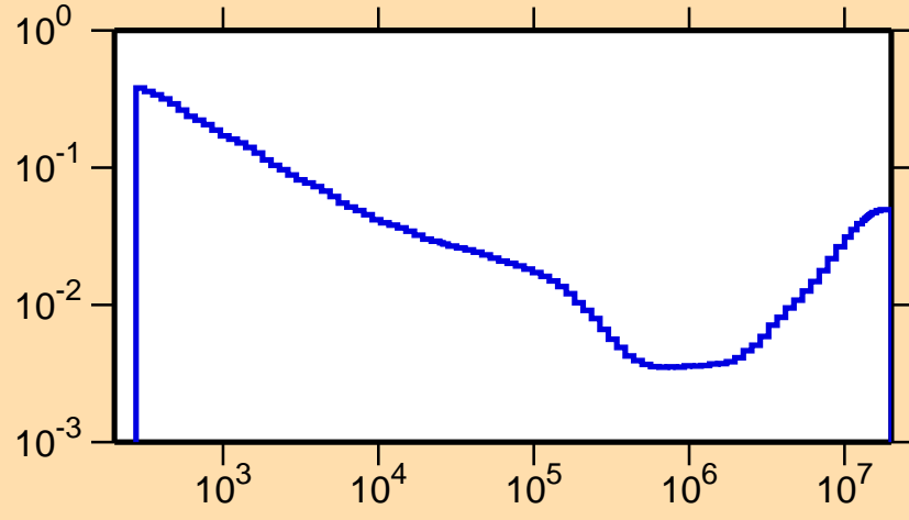
\sigma vs. E for ^{134}\text{La}(n,p)
