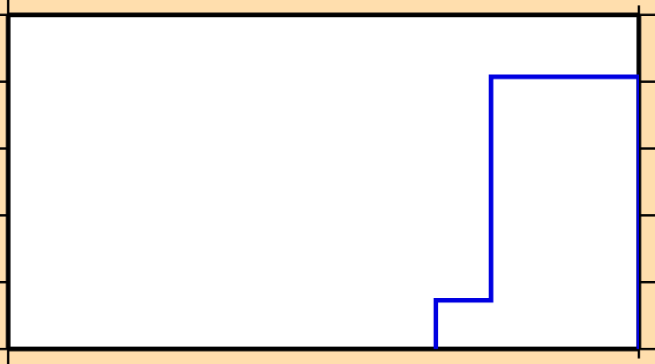
\sigma vs. E for ^{134}\text{La} (mt 34)
