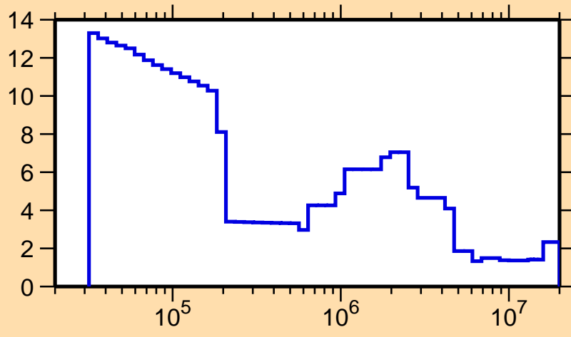
\Delta\sigma/\sigma vs. E for ^{134}\text{La}(n,\text{tot.})
