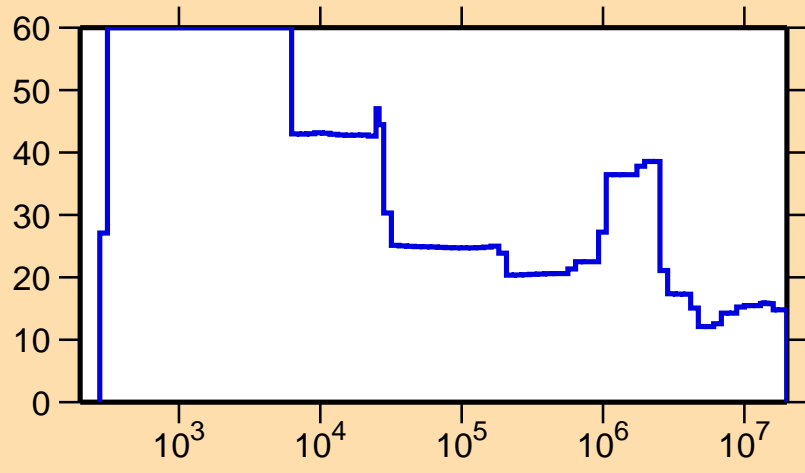
\Delta\sigma/\sigma vs. E for ^{134}\text{La}(n,p)
