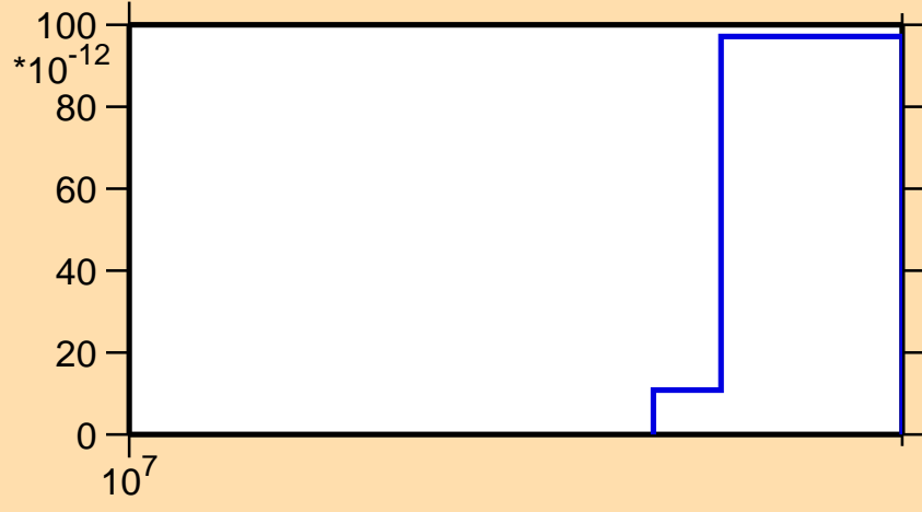
\sigma vs. E for ^{134}\text{La} (mt117)
