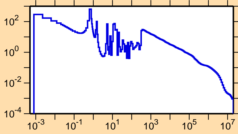
\sigma vs. E for ^{134}\text{La}(n,\gamma)
