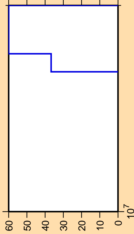
\Delta\sigma/\sigma vs. E for ^{134}\text{La} (mt117)
