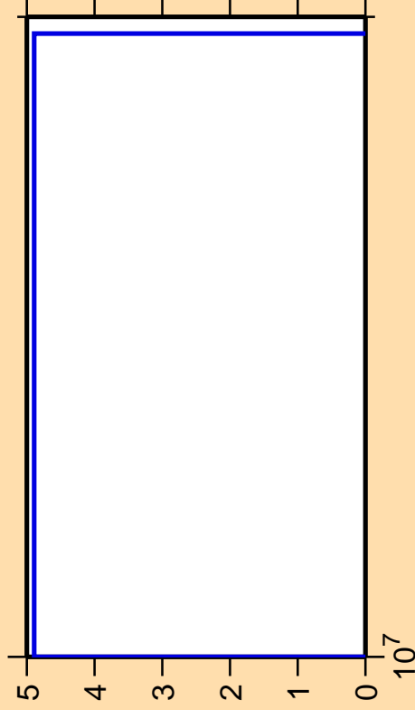
\Delta\sigma/\sigma vs. E for ^{134}\text{La}(\text{mt117})
