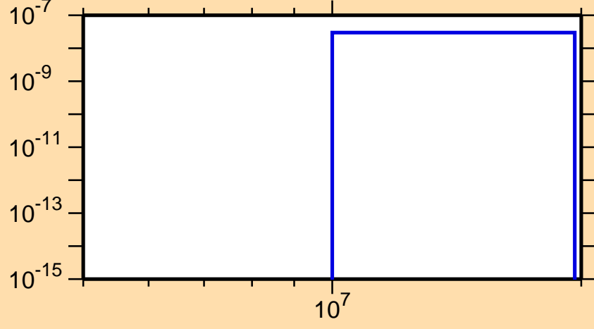
\sigma vs. E for ^{134}\text{La}(n,\text{He3})
