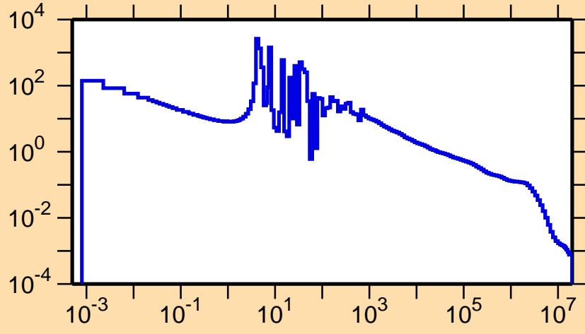
\sigma vs. E for ^{135}\text{La}(n,\gamma)
