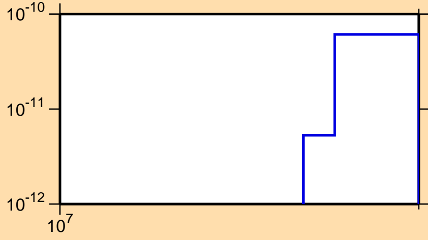
\sigma vs. E for ^{135}\text{La} (mt117)
