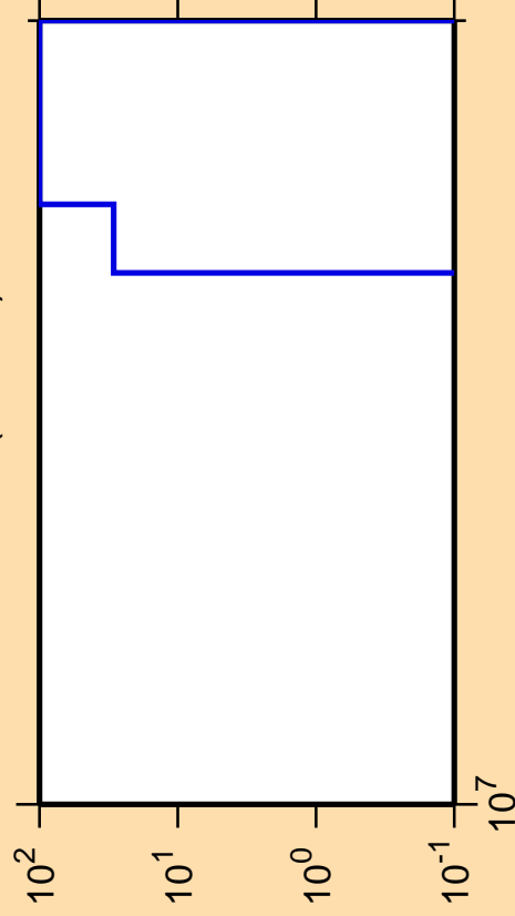
\Delta\sigma/\sigma vs. E for ^{135}\text{La} (mt117)
