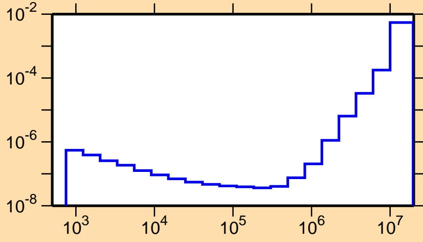
\sigma vs. E for ^{135}\text{La}(n,\alpha)
