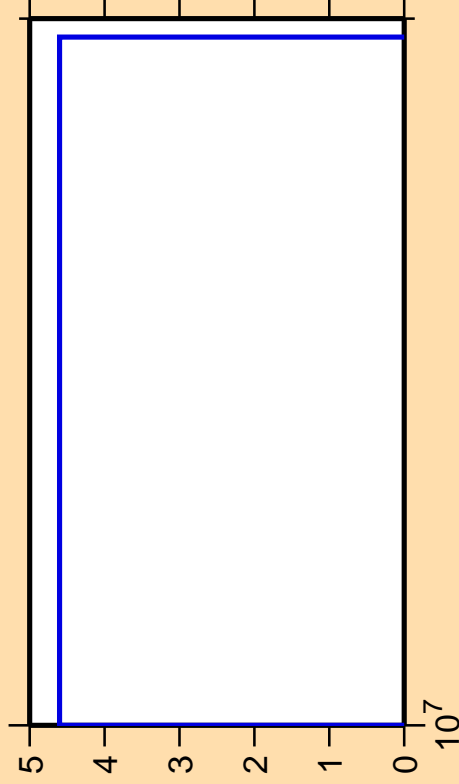
\Delta\sigma/\sigma vs. E for ^{135}\text{La}(\text{mt117})
