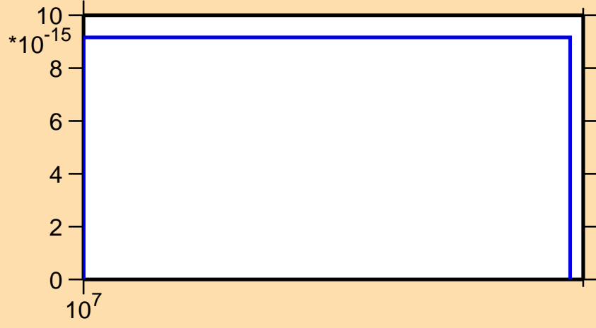
\sigma vs. E for ^{135}\text{La}(n,pd)
