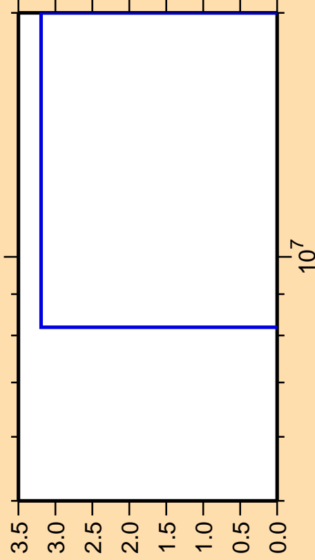
\Delta\sigma/\sigma vs. E for ^{135}\text{La} (mt 45)
