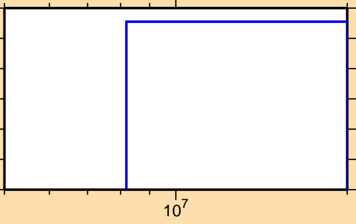
\sigma vs. E for ^{135}\text{La}(n,nt)
