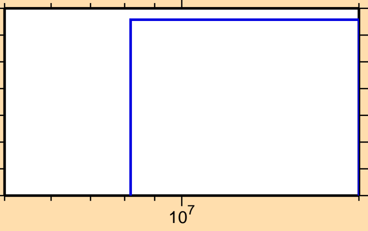
\sigma vs. E for ^{135}\text{La}(n,2np)
